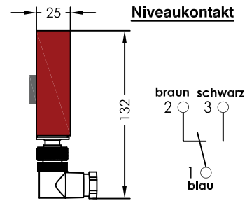
NRAC-W - M12
